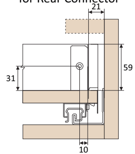
Installation Dimensions for Rear Connector
