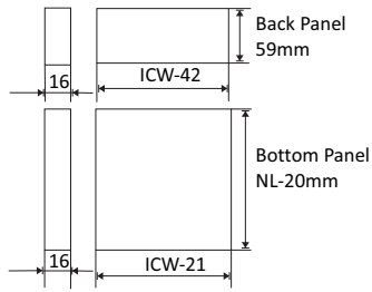
Space requirement in cabinet
