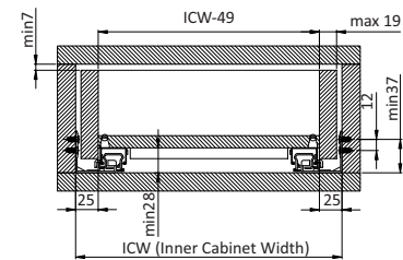
Installation for drawer with max. 19mm side
