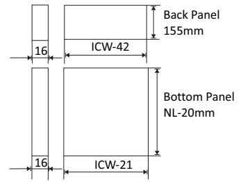
Installation Dimensions for Rear Connector
