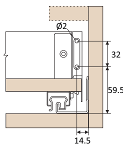
Installation Dimensions for Front Connector
